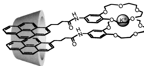
Fig. 1. Possible structure of 2:1:1 complex of C3-15C5 with \text{K}^+ and \gamma -CyD.
