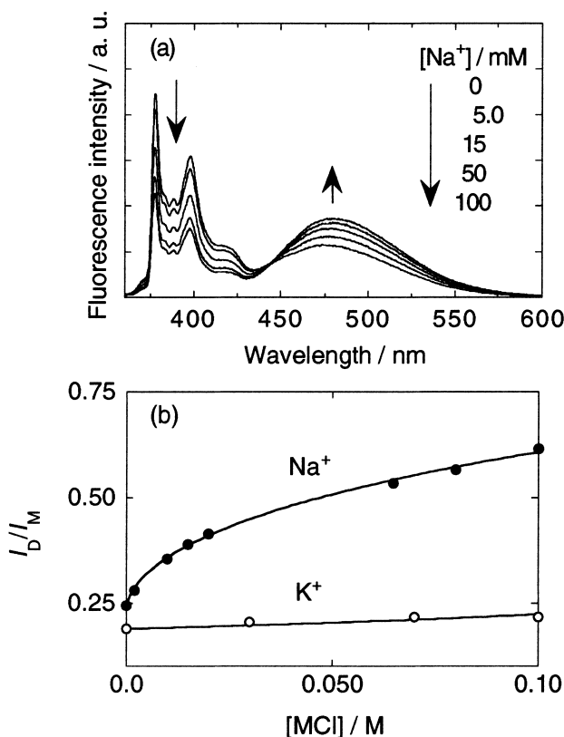
Fig. 5. (a) Fluorescence spectra of C3-12C4 . [ C3-12C4 ] = 0.50 μM in 99% water/1% MeCN (v/v); [γ-CyD] = 15 mM. Excitation wavelength: 331.0 nm. (b) Dependence of I_D/I_M on the concentration of (●) \text{Na}^+ and (○) \text{K}^+ . The emission wavelengths for the dimer/monomer fluorescence are 480/377 nm.
