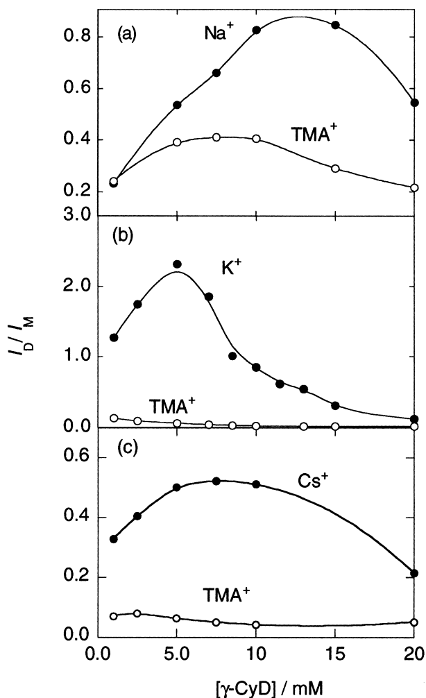
Fig. 4. Fluorescence intensity ratio, I_D/I_M , of (a) C3-12C4 , (b) C3-15C5 , and (c) C3-18C6 with 0.10 M (○) TMACl and 0.10 M (●) MCl as a function of \gamma -CyD concentration. [probe] = 0.50 \mu\text{M} in 99% water/1% MeCN (v/v). The guest cation and emission wavelengths for the dimer/monomer fluorescence are (a) \text{Na}^+ , 480/377 nm, (b) \text{K}^+ , 470/378 nm, and (c) \text{Cs}^+ , 470/377 nm, respectively.
