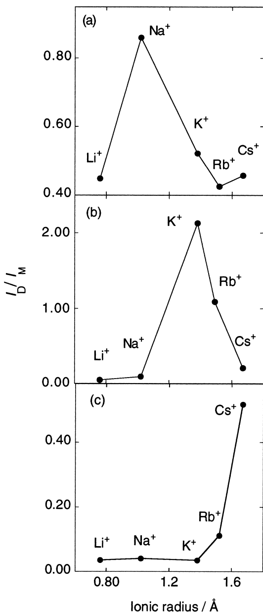
Fig. 3. Dependence of fluorescence intensity ratio, I_D/I_M , of (a) C3-12C4 , (b) C3-15C5 , and (c) C3-18C6 on the ionic radius of alkali metal ions. [probe] = 0.50 \mu\text{M} in 99% water/1% MeCN (v/v). [ \gamma -CyD] = 5.0 mM. [MCl] = 0.10 M ( \text{M}^+ = \text{Li}^+ , \text{Na}^+ , \text{K}^+ , \text{Rb}^+ , \text{Cs}^+ ). The emission wavelengths for the dimer/monomer fluorescence are (a) 480/377 nm, (b) 470/378 nm, and (c) 470/377 nm, respectively.
