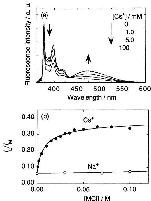
Fig. 6. (a) Fluorescence spectra of C3-18C6 . [ C3-18C6 ] = 0.50 μM in 99% water/1% MeCN (v/v). [γ-CyD] = 5.0 mM. Excitation wavelength: 329.0 nm. (b) Dependence of I_D/I_M on the concentration of (●) \text{Cs}^+ and (○) \text{Na}^+ . The emission wavelengths for the dimer/monomer fluorescence are 470/377 nm.
