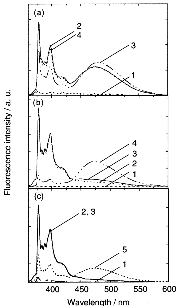
Fig. 2. Fluorescence spectra of probes ([probe] = 0.50 \mu M in 99% water/1% MeCN (v/v)) with added species. (a) C3-12C4 excited at 331.0 nm, (b) C3-15C5 excited at 330.5 nm and (c) C3-18C6 excited at 329.0 nm. (1) [ \gamma -CyD] = 0 mM and 0.10 M TMAcI. (2) [ \gamma -CyD] = 5.0 mM and 0.10 M TMAcI. (3) [ \gamma -CyD] = 5.0 mM and 0.10 M NaCl. (4) [ \gamma -CyD] = 5.0 mM and 0.10 M KCl. (5) [ \gamma -CyD] = 5.0 mM and 0.10 M CsCl.
